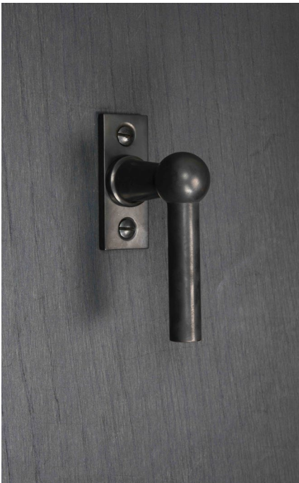
CDF-1814DK Retaise Length 85mm Projection 55mm
