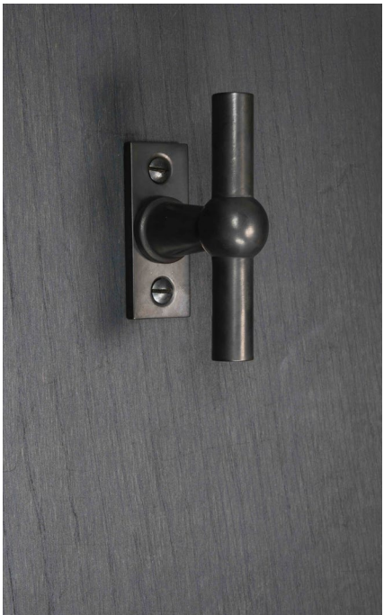
CDF-1814TDK Retaise Length 88mm Projection 55mm
