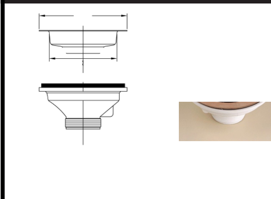
Drain Basket/ Crepine H45.21.X
