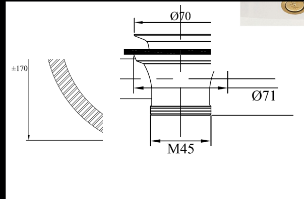
Drain Basket/ Crepine H45.09.X
