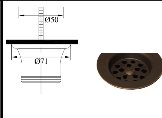
Drain Basket/ Crepine H45.05.X
